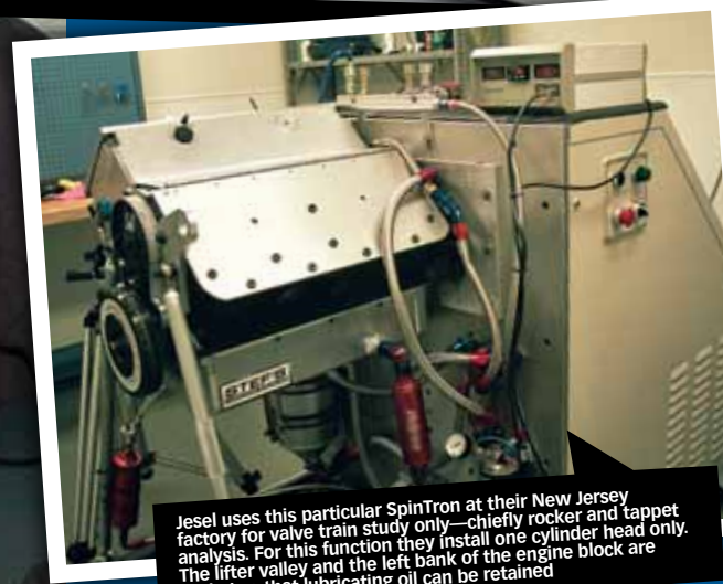
The normal lubrication system supplied with the SpinTron comprises: dry-sump oil reservoir, remote oil filter, and oil hoses. An oil pump is also included but not the oil pan. To maintain engine block rigidity, Spintron recommends no more than one cylinder opening per side, in contrast to the engine displayed
